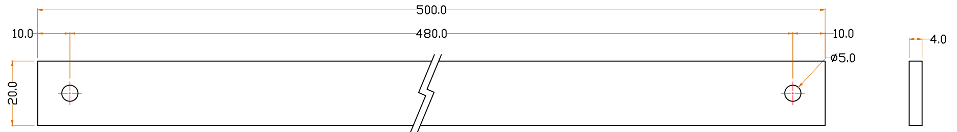
FRONT VIEW
