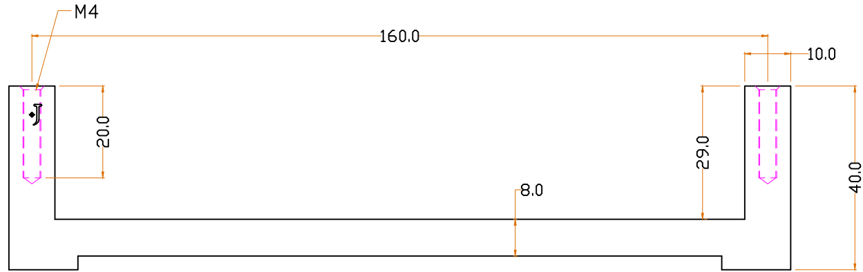
TOP VIEW
