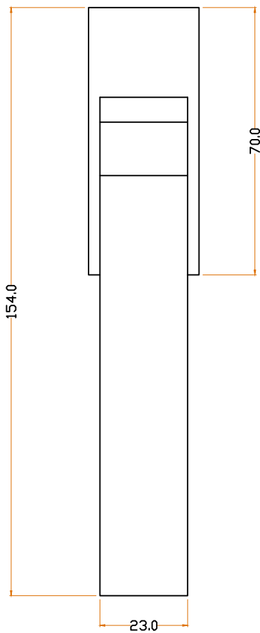
FRONT VIEW
